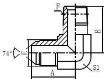
NPT MALE
